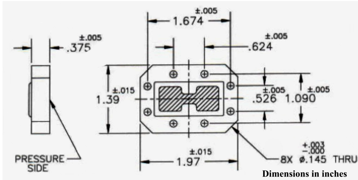
Broadband teflon fiberglass window for use in double ridge waveguide
